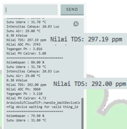
Gambar IV.7 Kalibrasi Sensor TDS
