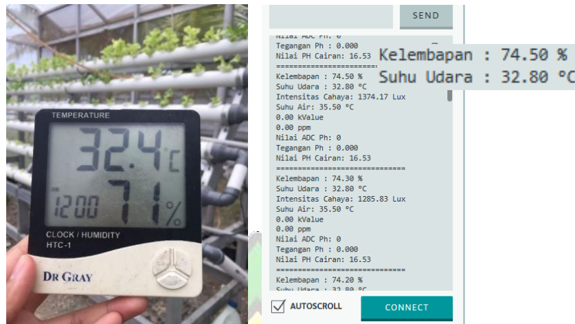
Gambar IV.4 Kalibrasi Sensor DHT22
