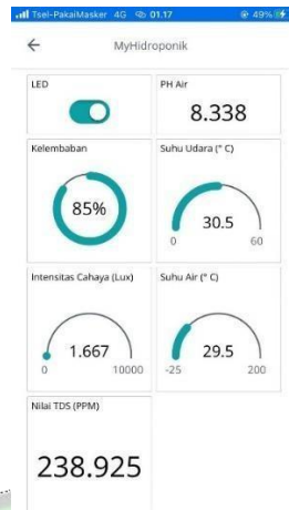
Gambar IV.3 Dashboard Arduino Cloud Remote
