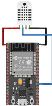
Gambar III.2 Rangkaian Sensor DHT22
