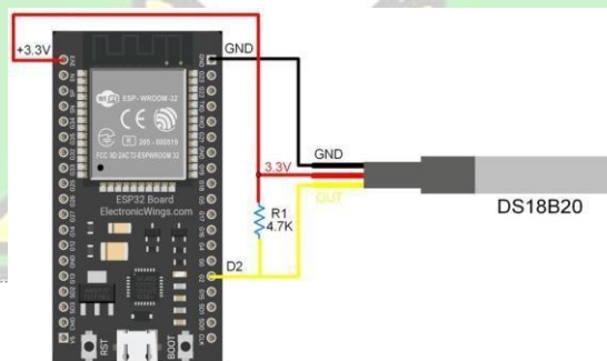
Gambar III.3 Rangkaian Sensor DS18B20
