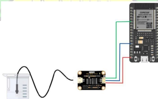
Gambar II.5 Rangkaian Sensor TDS
