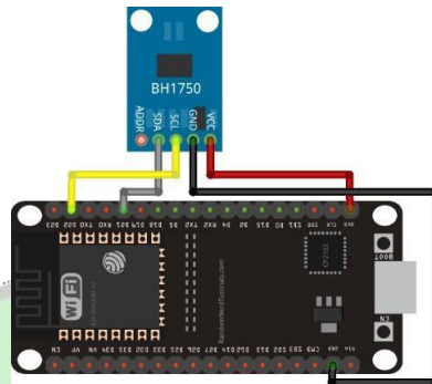
Gambar III.4 Rangkaian Sensor BH1750
