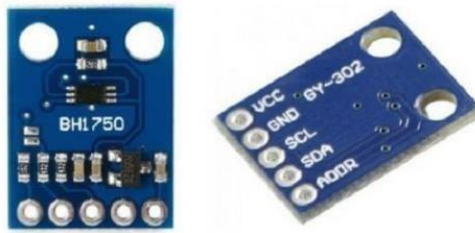
Gambar II.7 Sensor BH1750 (Suryana, 2021)
