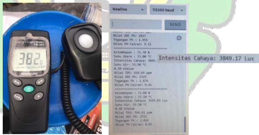
Gambar IV.6 Kalibrasi Sensor BH1750
